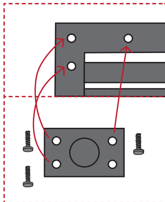
Method for installing the corner legs
