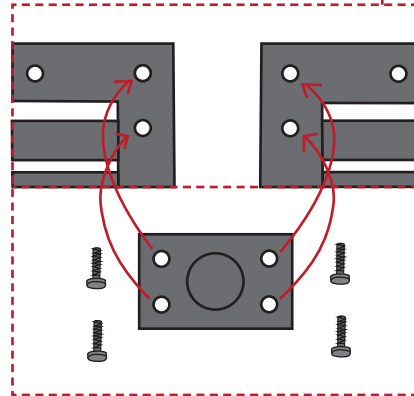
Method for installing the middle legs
